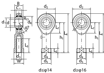
PHS - Rod end requiring maintenance with grease nipple and grease groove
